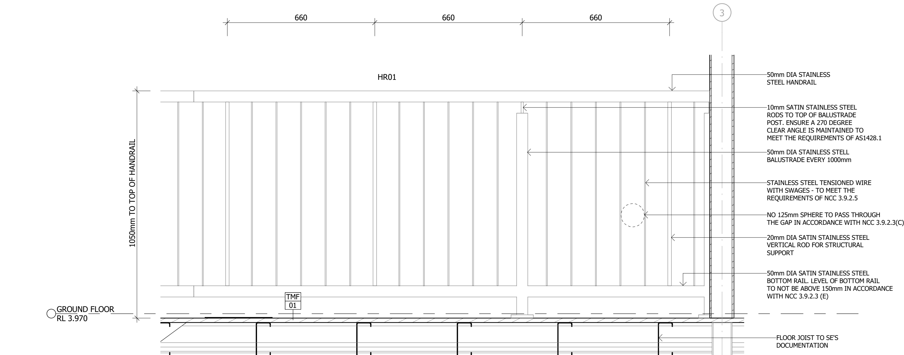
5 BALUSTRADE ELEVATION 1 : 10
